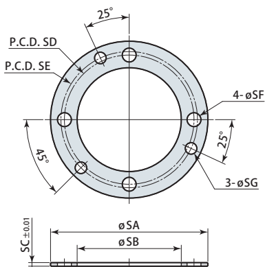
Shim (option)
