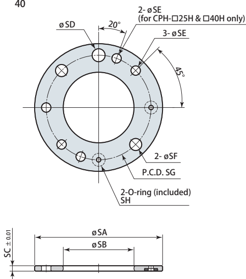
Shim (option)
