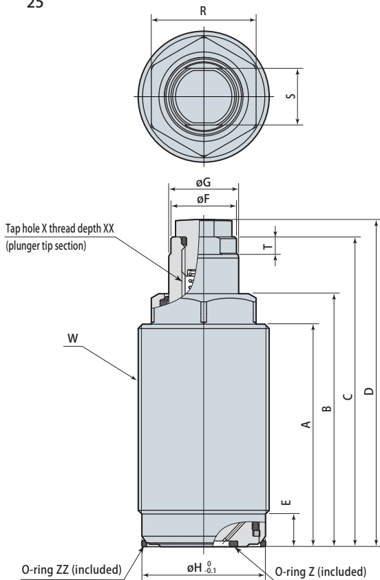
Mounting details
