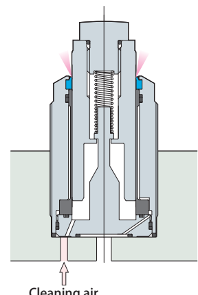
Recommended cleaning air pressure 0.3 ~ 0.5 MPa
