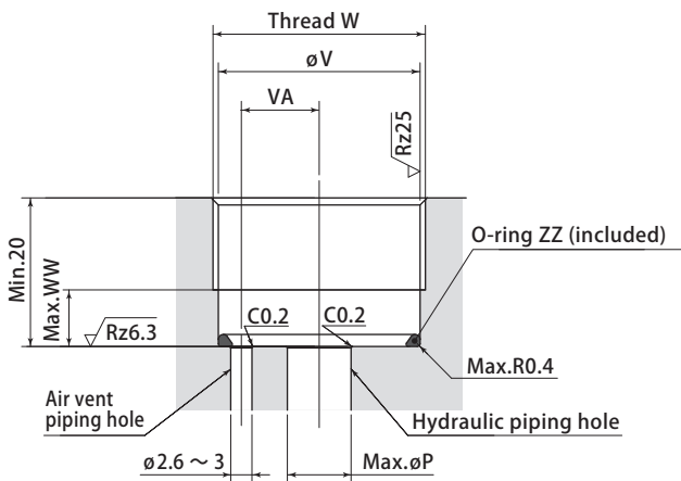
Mounting details
