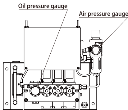
Control unit HCSD-H2EDDD
