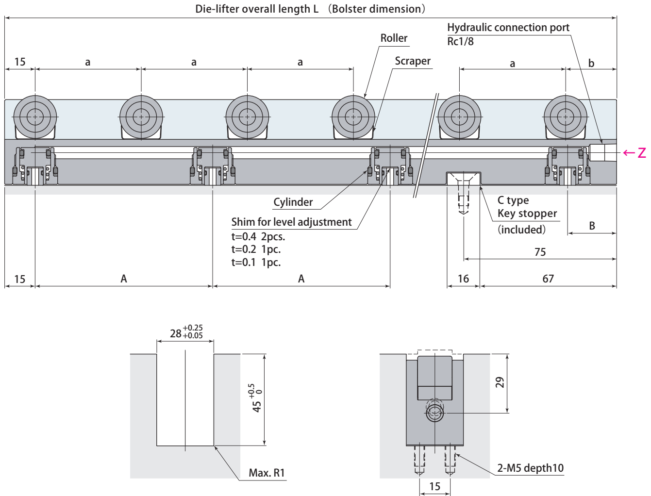
Slot details
