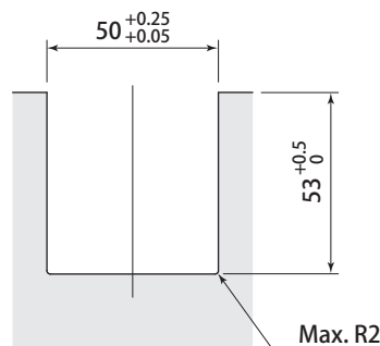
Slot details
