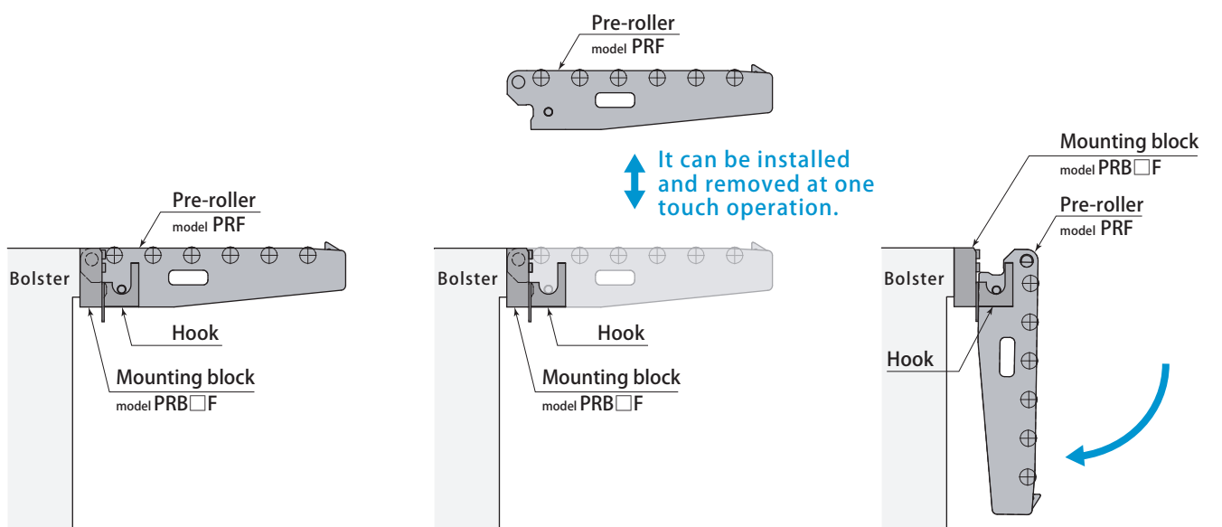
At hanging
