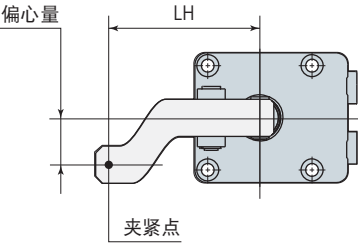
偏心型夹紧臂
